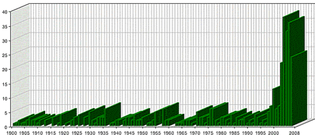
USGS Worldwide Deadly & Destructive Earthquakes of magnitude 6 or higher (1900-2008)
